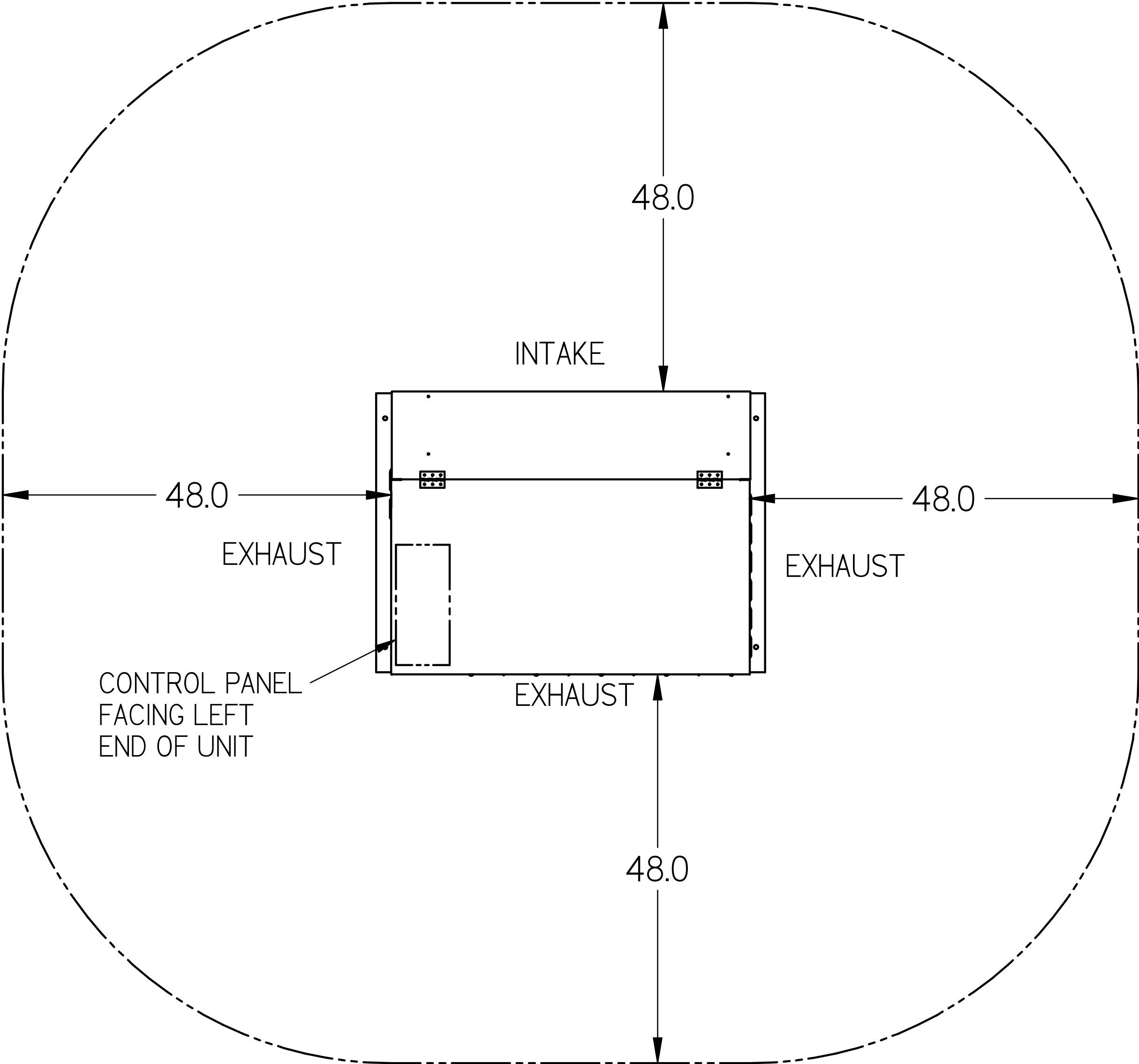
CLEARANCE ON A SINGLE UNIT APPLICATION
