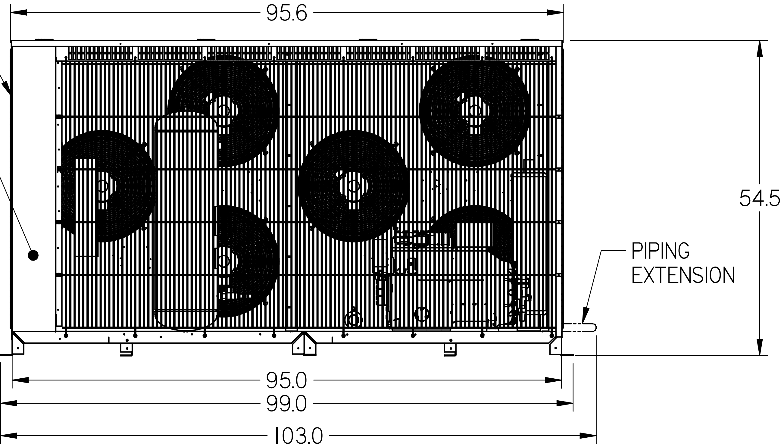
FRONT VIEW
