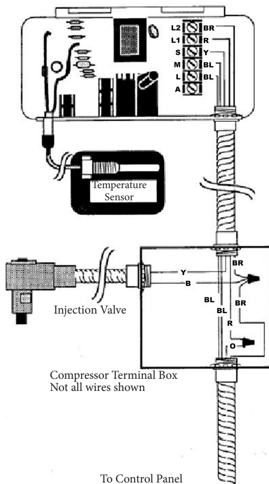
Figure 2-11 Demand Cooling Wiring
