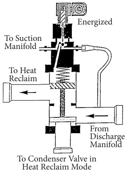
Figure 2-8 Heat Reclaim Valve Heat Reclaim Mode
