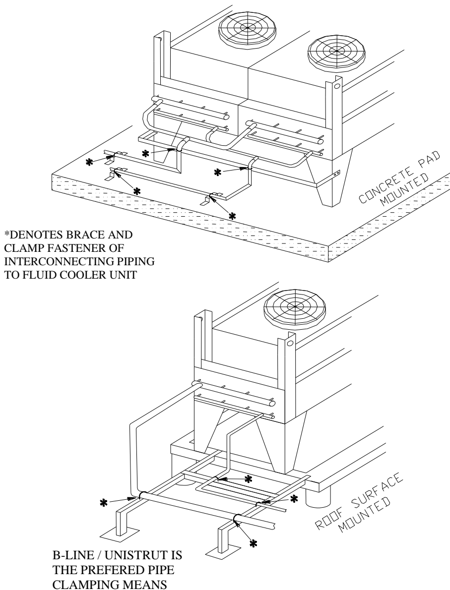
FIGURE 8 UNIT MOUNTING AND PIPING
