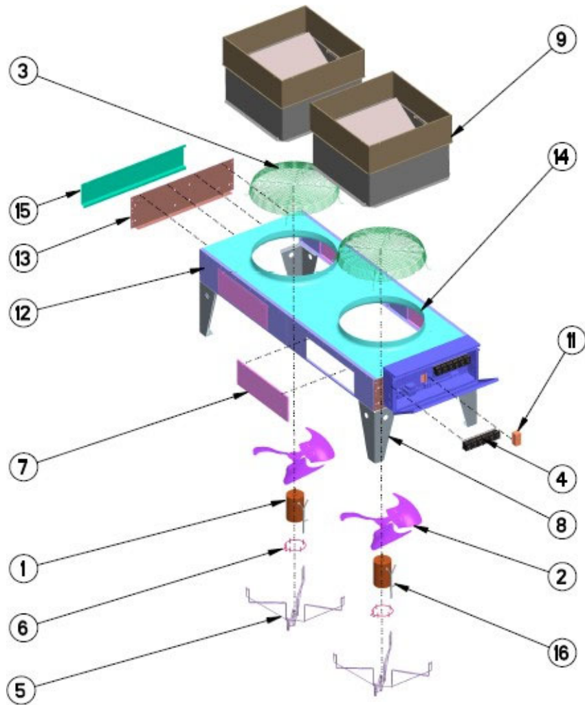
Figure 263 - REPLACEMENT PARTS
